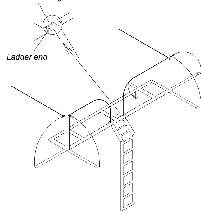
Ladder Mounting Guide - Bend Down
